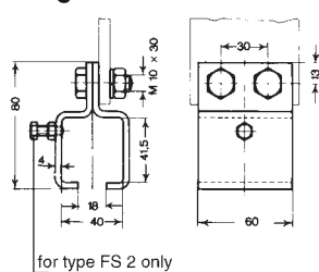
Hanger lateral
