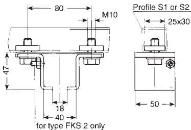
Hanger unterhung for HK support
